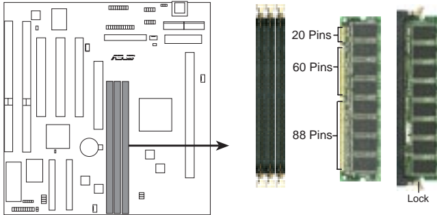
P2L-B 168 Pin DIMM Memory Sockets
