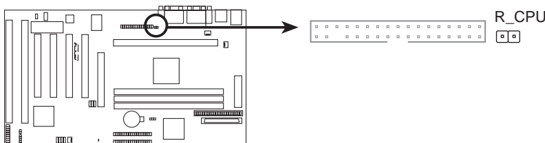
P2L97-S CPU Thermal Sensor Connector
