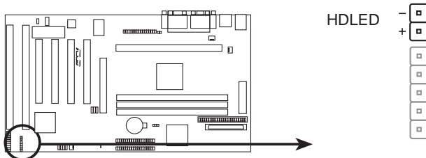
P2L97-S Hard Disk Activity LED
