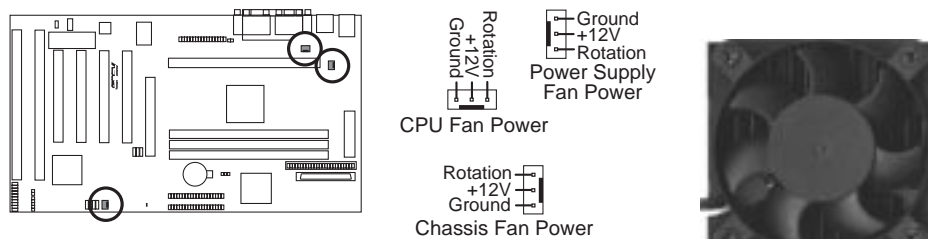
P2L97-S 12Volt Cooling Fan Power
