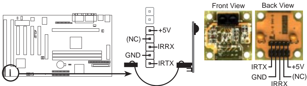
P2L97-S Infrared Module Connector
