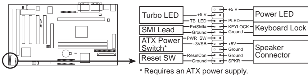
P2L97-S System Panel Connections
