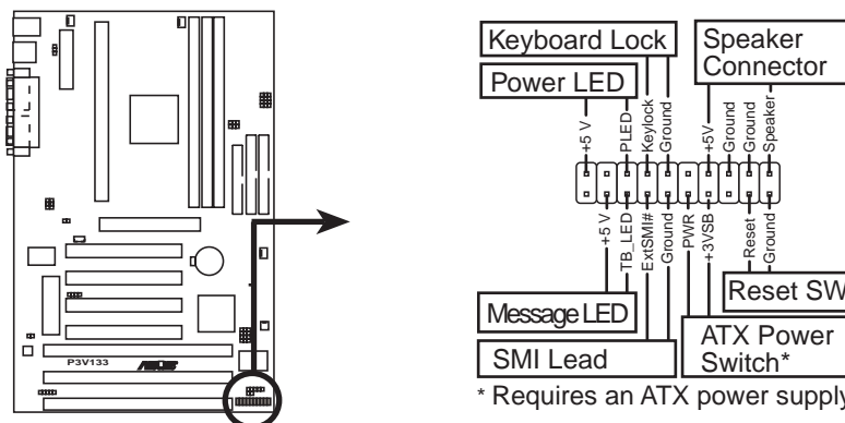
P3V133 System Panel Connections
