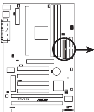
P3V133 Floppy Disk Drive Connector
