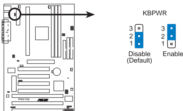
P3V133 Keyboard Power Up
