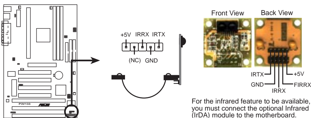
P3V133 Infrared Module Connector
