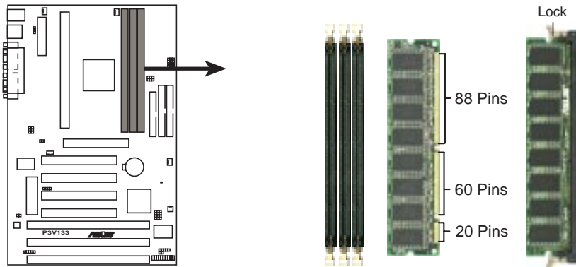
P3V133 168-Pin DIMM Memory Sockets
