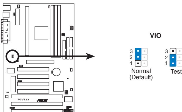
P3V133 Input/Output Voltage Selection
