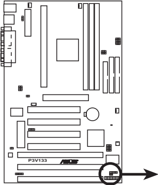
P3V133 IDE Activity LED
