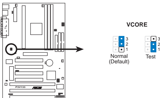
P3V133 CPU Core Voltage Selection
