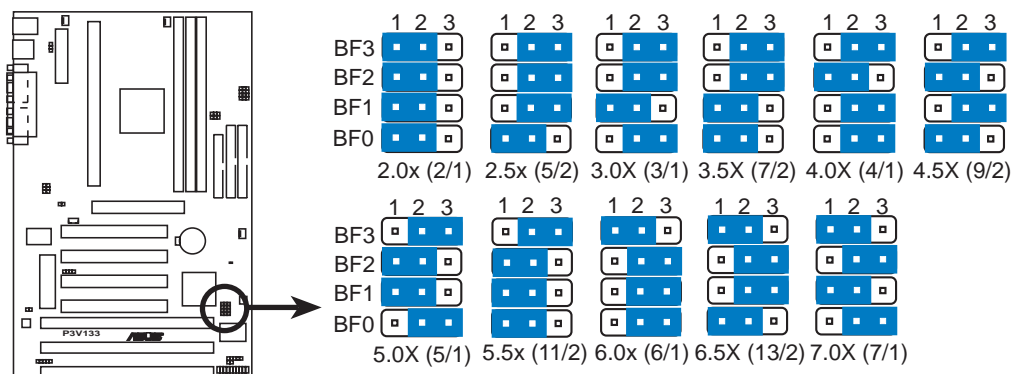
P3V133 CPU Core:BUS Frequency Multiple
