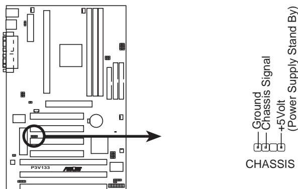
P3V133 Chassis Open Alarm Lead
