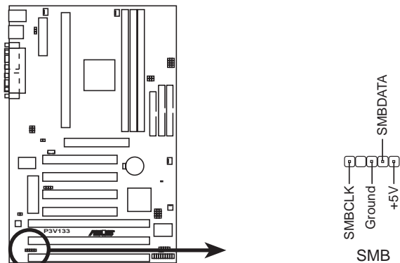
P3V133 SMBus Connector
