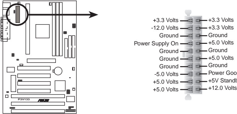
P3V133 ATX Power Connector
