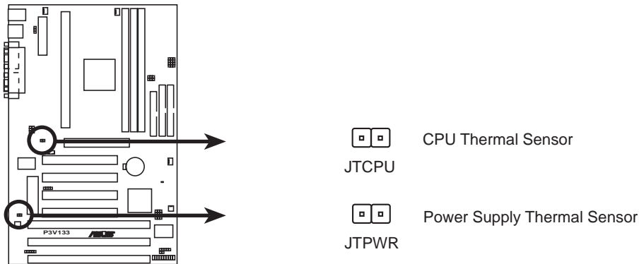
P3V133 Thermal Sensor Connectors
