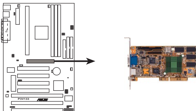
P3V133 Accelerated Graphics Port (AGP)
