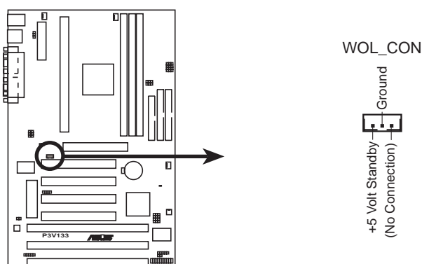
P3V133 Wake on LAN Connector
