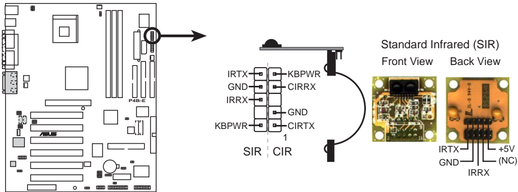
P4B-E Infrared Module Connector
