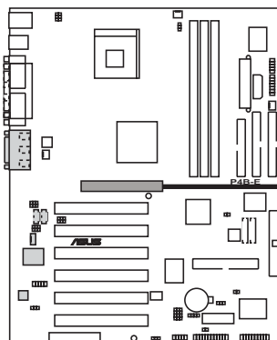
P4B-E Accelerated Graphics Port (AGP)
