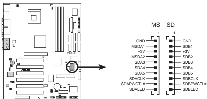
P4B-E MS/SD Connectors
