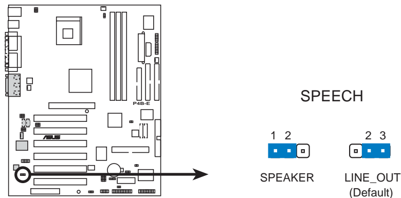
P4B-E Speaker Selector
