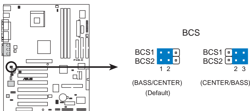
P4B-E Bass Center Setting
