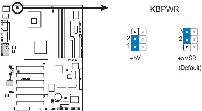
P4B-E Keyboard Power Setting
