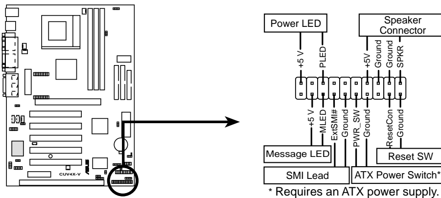
CUV4X-V System Panel Connectors
