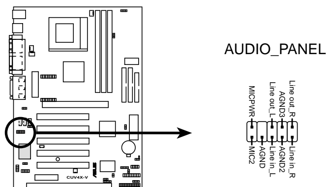
CUV4X-V Audio Panel Connectors
