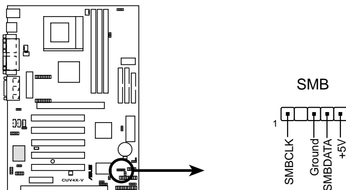
CUV4X-V SMBus Connector
