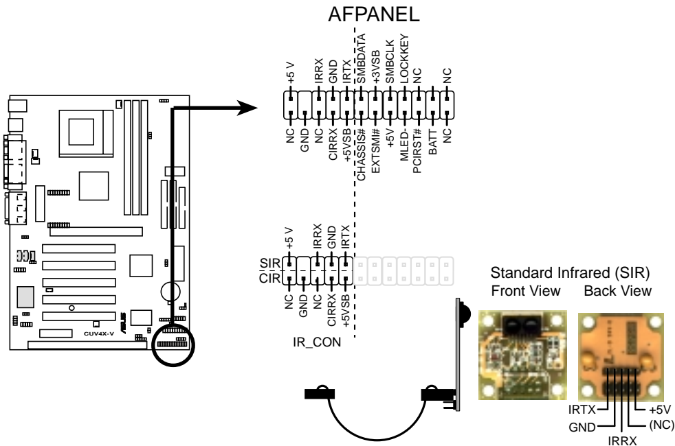
CUV4X-V Front Panel Connectors
