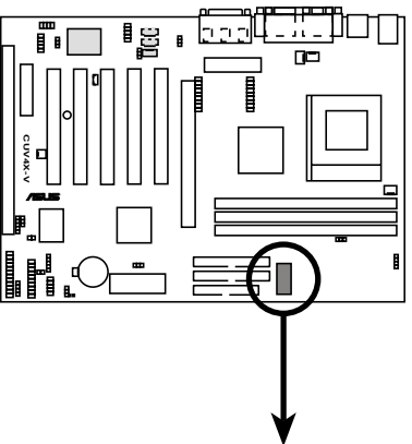
CUV4X-V DIP Switches
