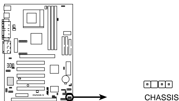
CUV4X-V Chassis Open Alarm Lead
