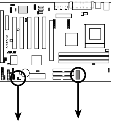
CUV4X-V JumperFree™ Mode Setting
