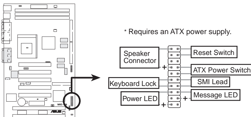
ME-99 System Panel Connectors
