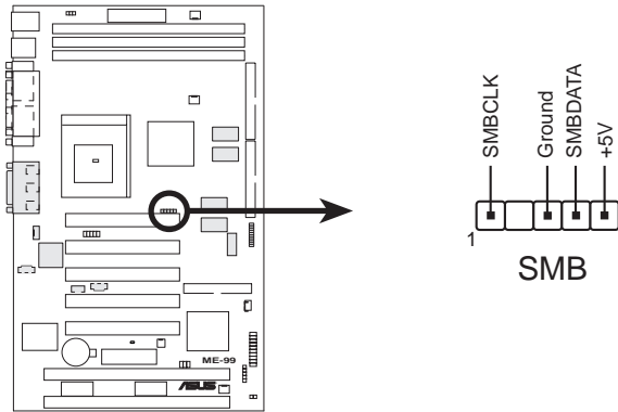
ME-99 SMBus Connector
