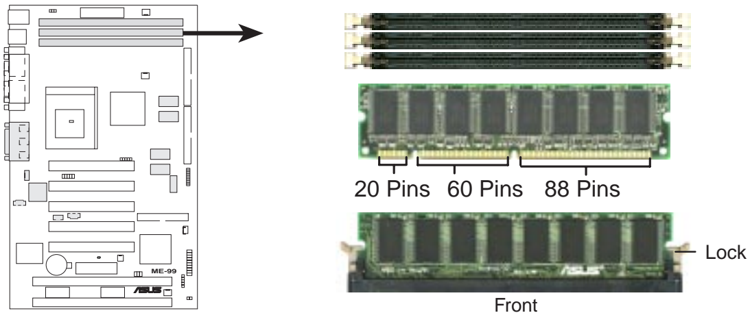
ME-99 168-Pin DIMM Sockets
