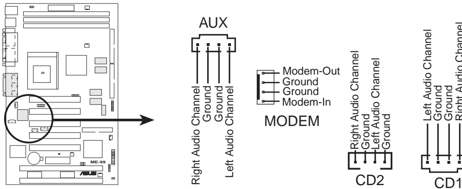
ME-99 Internal Audio Connectors
