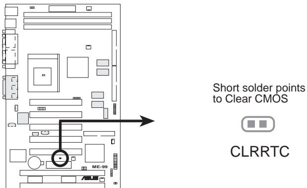
ME-99 Clear RTC RAM
