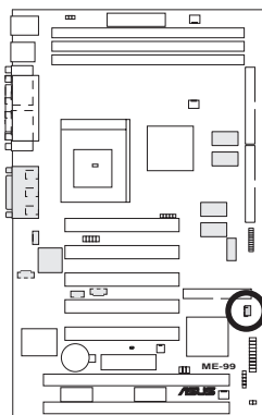
ME-99 Wake-On-LAN Connector
