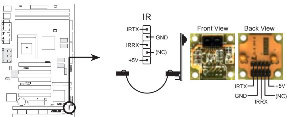
ME-99 Infrared Module Connector
