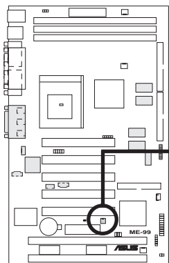
ME-99 Wake-On-Ring Connector
