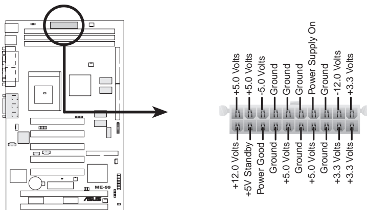
ME-99 ATX Power Connector
