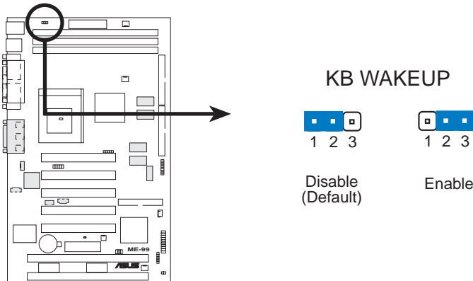
ME-99 Keyboard Wake Up
