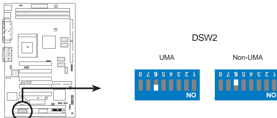
ME-99 VGA Frame Buffer Setting
