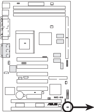
ME-99 IDE Activity LED
