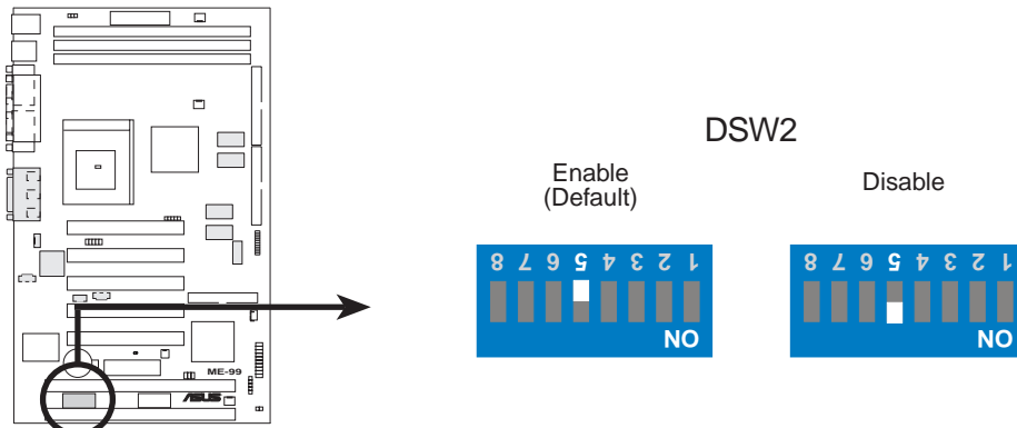
ME-99 Onboard VGA Setting
