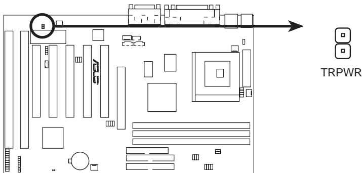
P5A Power Supply Temperature External Connector
