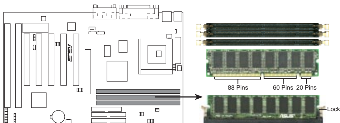
P5A 168 Pin DIMM Memory Sockets
