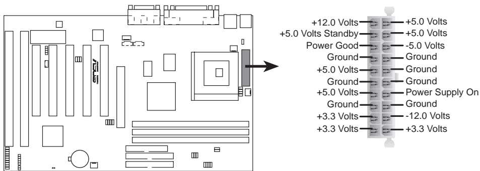
P5A ATX Power Connector
