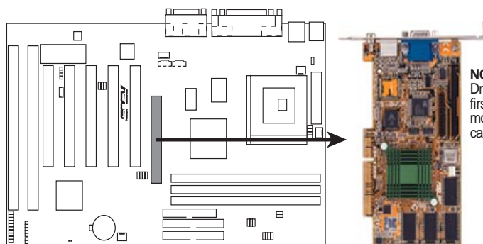
P5A Accelerated Graphics Port (AGP)
