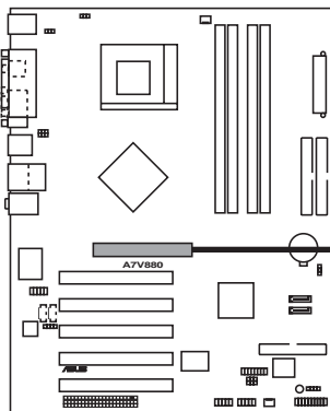
A7V880 Accelerated Graphics Port (AGP)
