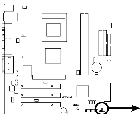
A7V-M Wake-On-Ring-Connector
