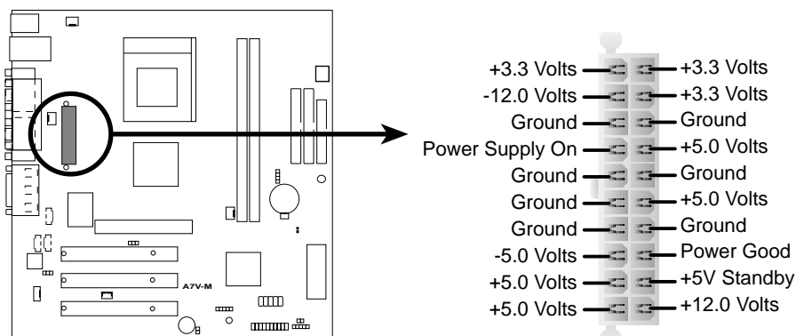
A7V-M ATX Power Connector
