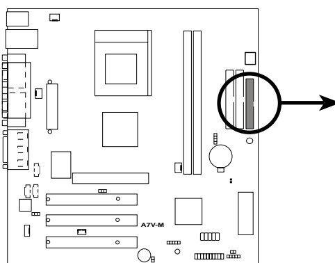
A7V-M Floppy Disk Drive Connector
