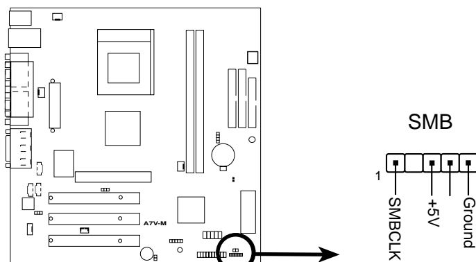
A7V-M SMBus Connector
