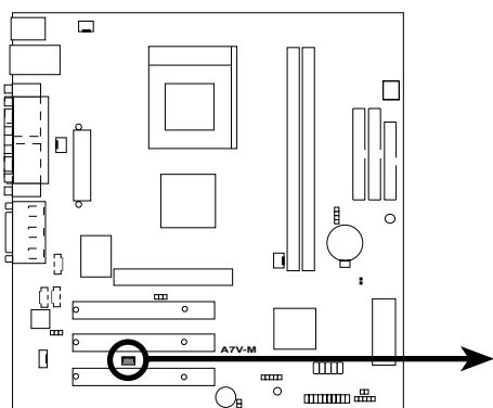
A7V-M Wake-On-LAN Connector
