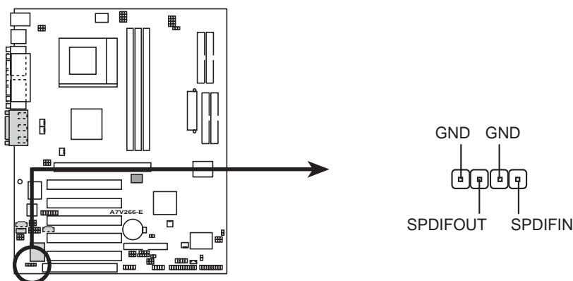
A7V266-E Digital Audio Interface
