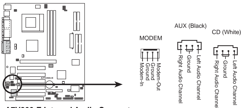
A7V266-E Internal Audio Connectors
