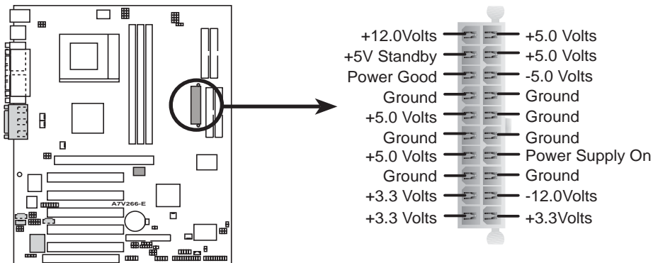
A7V266-E ATX Power Connector
