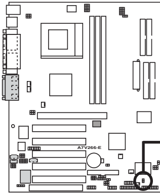
A7V266-E IDE Activity LED
