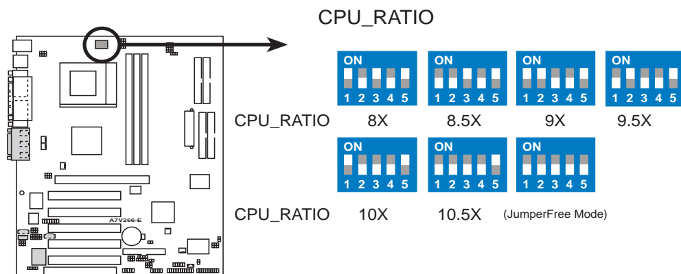
A7V266-E CPU External Clock (BUS) Frequency Selection
