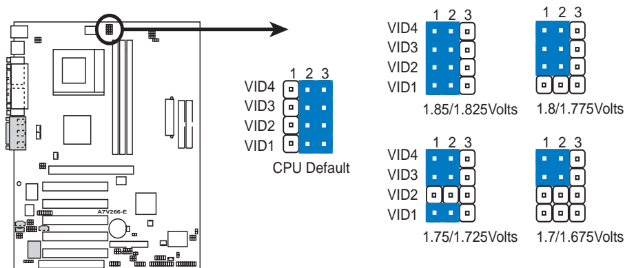
A7V266-E CPU Core Voltage Selection
