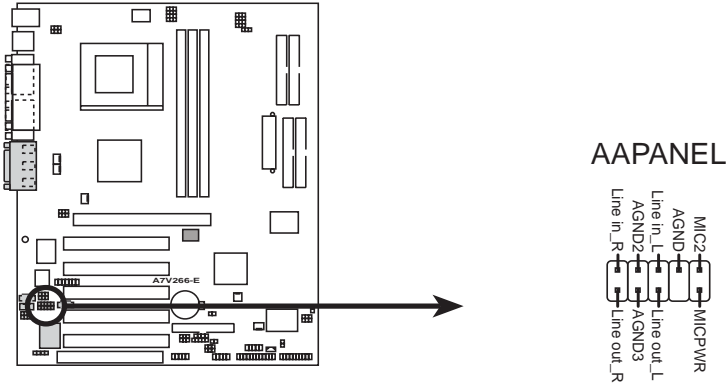
A7V266-E Audio Panel Connectors
