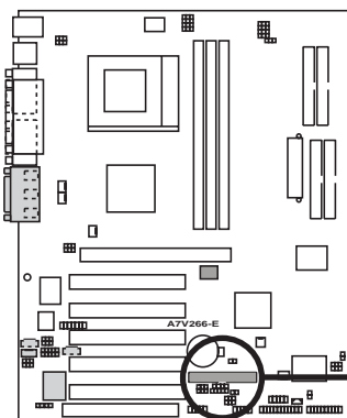
A7V266-E Floppy Disk Drive Connector
