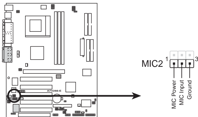
A7V266-E Internal Microphone Connector
