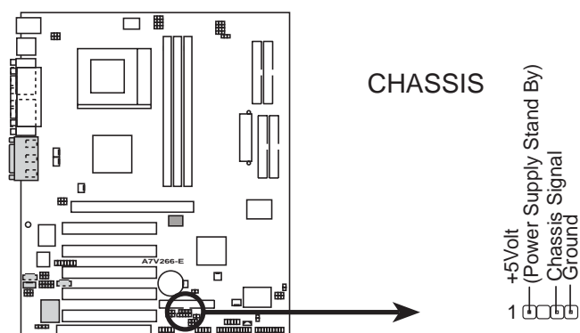
A7V266-E Chassis Open Alarm Lead
