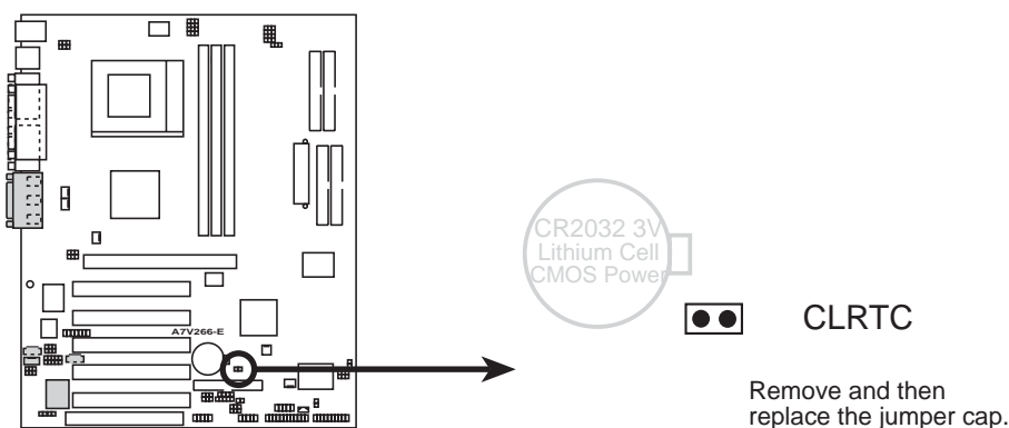
A7V266-E Clear RTC RAM
