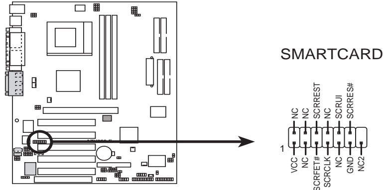
A7V266-E Smartcard
