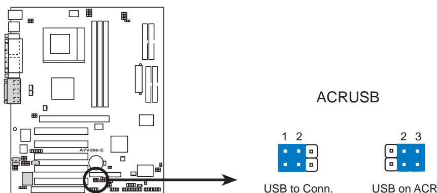
A7V266-E USB/ACR Selection
