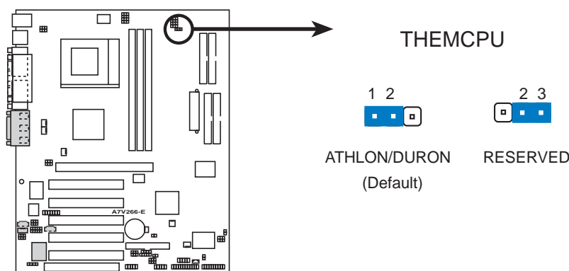
A7V266-E THEMCPU Setting
