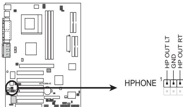
A7V266-E True-Level Line Out Header
