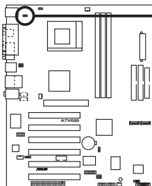
A7V600 Keyboard Power Setting
