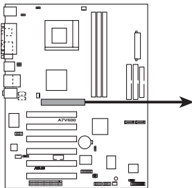
A7V600 Accelerated Graphics Port (AGP)
