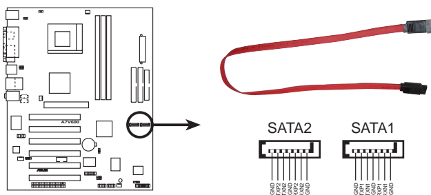
A7V600 SATA Connectors
