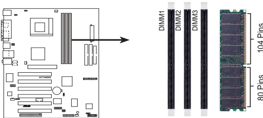
A7V600 184-Pin DDR DIMM Sockets
