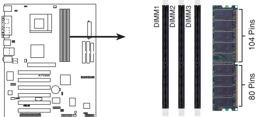
A7V600 184-Pin DDR DIMM Sockets
